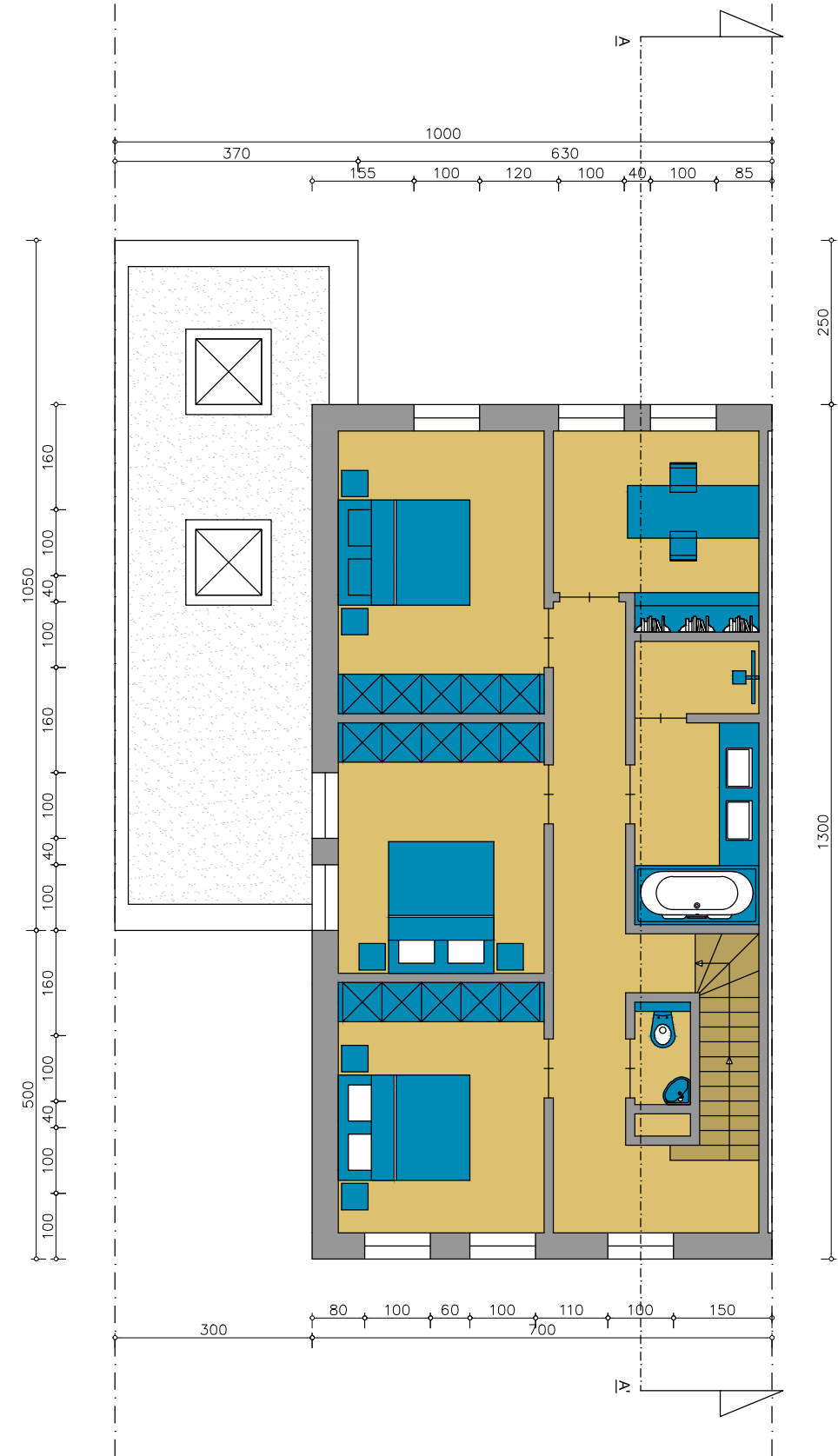
WONING TYPE 1 PLAN VERDIEPING +1
